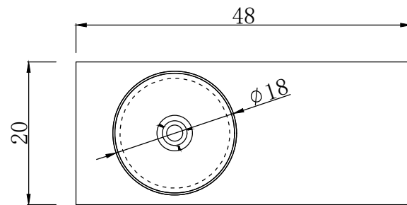
SINK TOP VIEW
