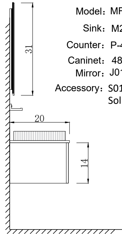
SIDE VIEW
